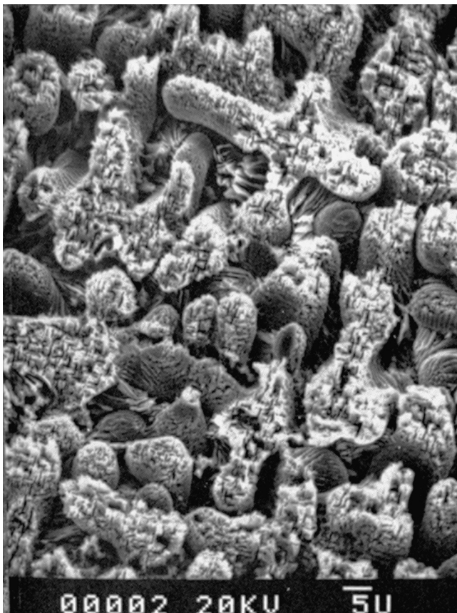
Fig. 25.16 Scanning electron micrograph of etched base metal ( \times 1000 ). (Courtesy of B. K. Moore.)
