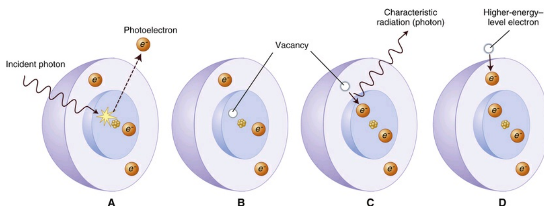
FIG. 1.22 Photoelectric absorption. (A) Photoelectric absorption occurs when an incident photon gives up all of its energy to an inner electron, which is ejected from the atom (a photoelectron). The incident electron ceases to exist at this point. (B) The ionized atom now has an electron vacancy in the inner orbital. (C) An electron from a higher energy level fills the vacancy and emits characteristic radiation. (D) All orbitals are subsequently filled, completing the energy exchange.
