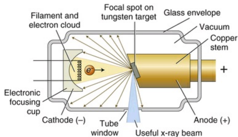
FIG. 1.6 X-ray tube with the major components labeled. The path of the electron beam is shown in yellow . X-rays produced at the target travel in all directions. The useful x-ray beam is shown in blue .
