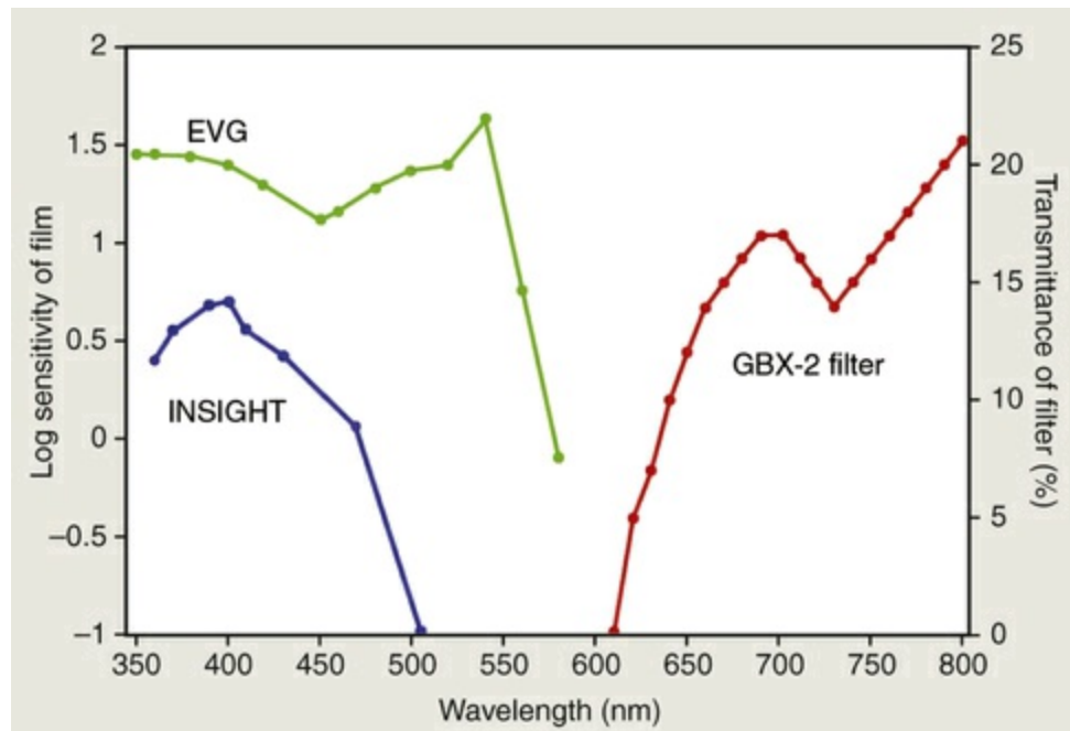
FIG. 5.17 Spectral sensitivities of EVG film (green line) and INSIGHT film (blue line) shown with the transmission characteristics of a GBX-2 filter (red line). The films are more sensitive in the blue-green portion of the spectrum (shorter than 600 nm), whereas the GBX-2 filter transmits primarily at the red end of the spectrum (longer than 600 nm).
