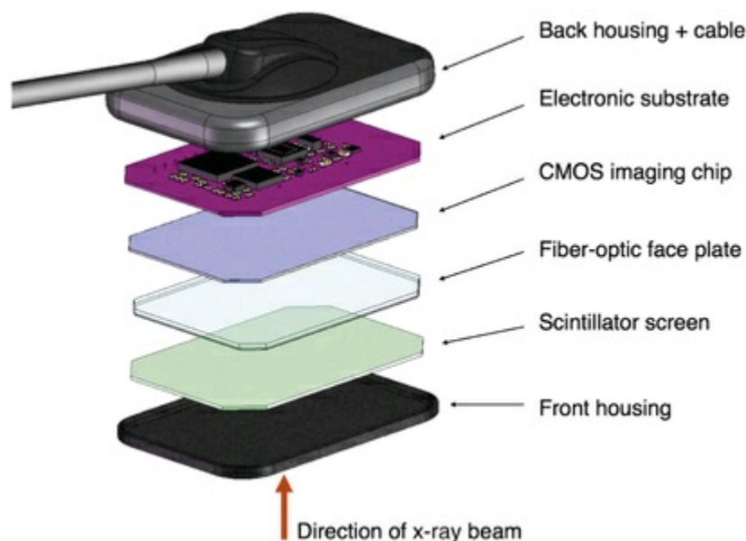
FIG. 4.3 Exploded View of Complementary Metal Oxide Semiconductor (CMOS) Sensor. The front and back housings form a watertight and light-tight barrier to protect the sensor components. The scintillator screen fluoresces when exposed to x-rays and forms a visible light radiographic image. The fiberoptic faceplate couples the scintillator screen to the CMOS chip to reduce image noise. The CMOS imaging chip captures the light from the scintillator and creates a charge in each pixel proportional to the exposure. The sensor electronics read the charge in each pixel and transmit it to a computer. (Courtesy XDR Radiology, Los Angeles, CA, https://www.xdradiology.com .)
