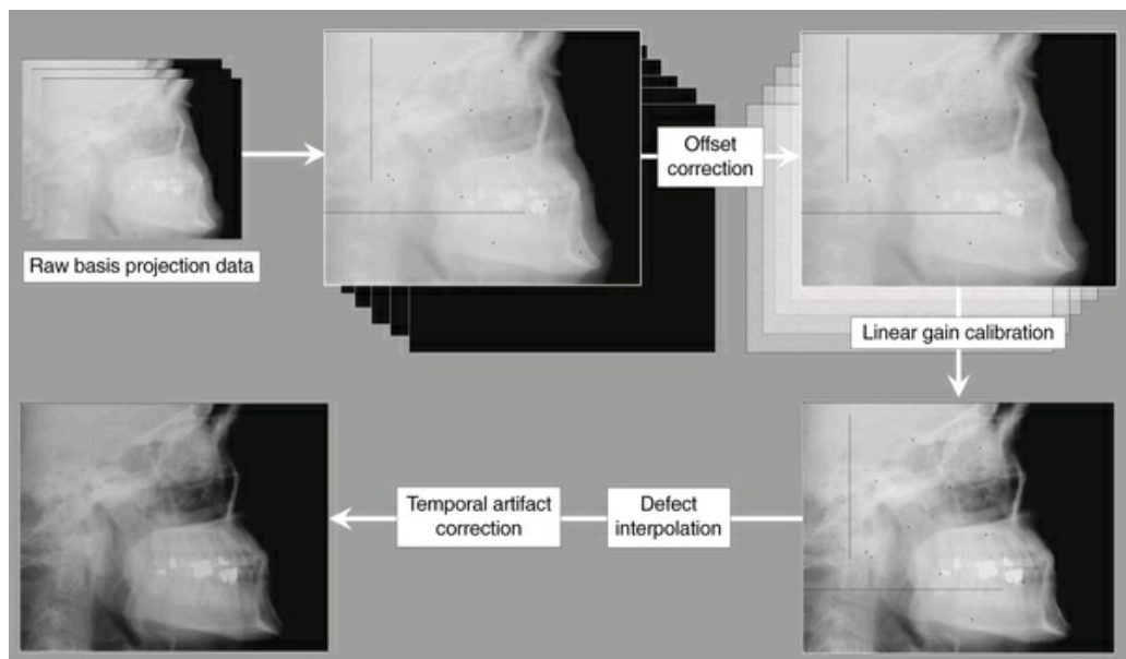
FIG. 10.8 Cone Beam Computed Tomography (CBCT) Detector Preprocessing. The first step of CBCT detector preprocessing is offset correction. This is accomplished by pixel-wise subtraction of an individual offset value computed by averaging over a series of up to 30 dark images. The second step is the linear gain calibration, consisting of dividing each pixel by its individual gain factor. The gain factors are obtained by averaging a sequence with up to 30 images of homogeneous exposures without any object between x-ray source and detector. The gain sequence is first offset corrected with its own sequence of dark images. The next procedure is the defect interpolation. Each pixel that shows unusual behavior, either in the gain image or in the average dark sequence, is marked in a defect map. The gray values of pixels classified as defective in this way are computed by linear interpolation along the least gradient descent. For flat panel detectors, there is usually an additional procedure to correct for temporal artifacts. These arise in such detectors because both the scintillator and the photodiodes exhibit residual signals.
