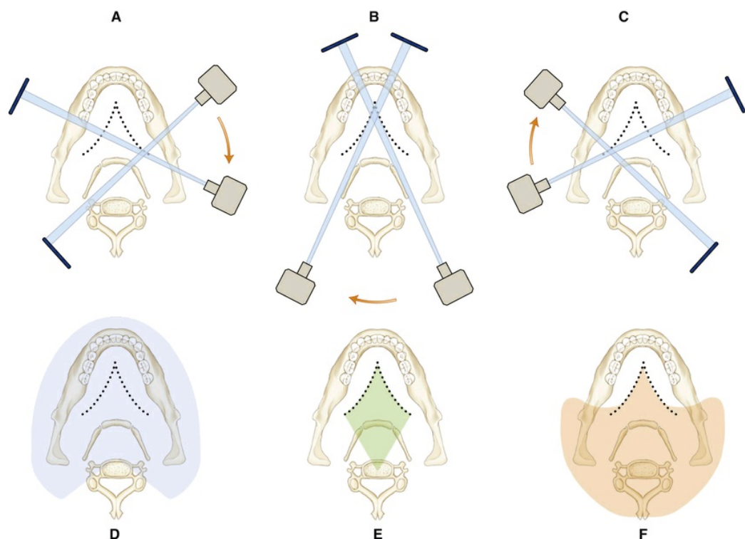
FIG. 9.8 Formation of real, double, and ghost images. (A–C) The exposure begins with the x-ray tube head on the patient's right side and continues with the tube head moving behind the patient and ending on the left side. The dotted line represents the path of the moving center of rotation during the exposure cycle. (D) Structures between the moving
