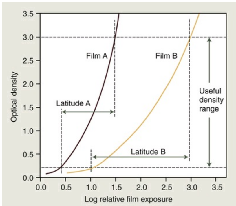
FIG. 5.28 Characteristic curves for two films demonstrating greater inherent latitude of film B compared with film A . The slope of film B is less steep than the slope of film A ; film B records a greater range of exposures within the useful density range than film A .
