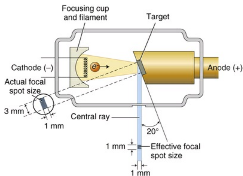
FIG. 1.8 The angle of the target to the central ray of the x-ray beam has a strong influence on the apparent size of the focal spot. The projected effective
