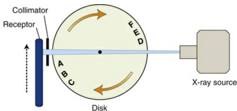
FIG. 9.3 Producing a panoramic image: In this conceptual view, the x-ray source and collimator are held stationary. The receptor moves through the beam, and the rotating disk also carries objects A–F through the beam. Objects A–C move through the beam at the same rate and direction as the image receptor and are imaged well. Objects D–F move through the beam at the same rate as the receptor but in the opposite direction, and so their images are blurred. The principles of panoramic image formation are the same for film-based and digital systems.
