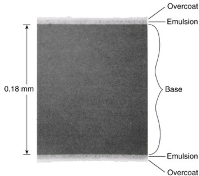
FIG. 5.1 Scanning electron micrograph of INSIGHT dental x-ray film (original magnification 300×). Note the overcoat, emulsion, and base on this double-emulsion film. (Courtesy Carestream Dental, a division of Carestream Health, Inc., Atlanta, Georgia.)
