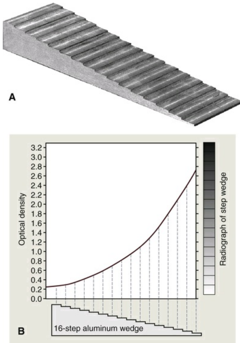
FIG. 5.22 (A) Aluminum step wedge. (B) Graph of the optical density of a radiograph made by exposing the step wedge. As the thickness of the aluminum decreases, more photons are passed through the wedge and are available to expose the film, and the image becomes progressively darker.
