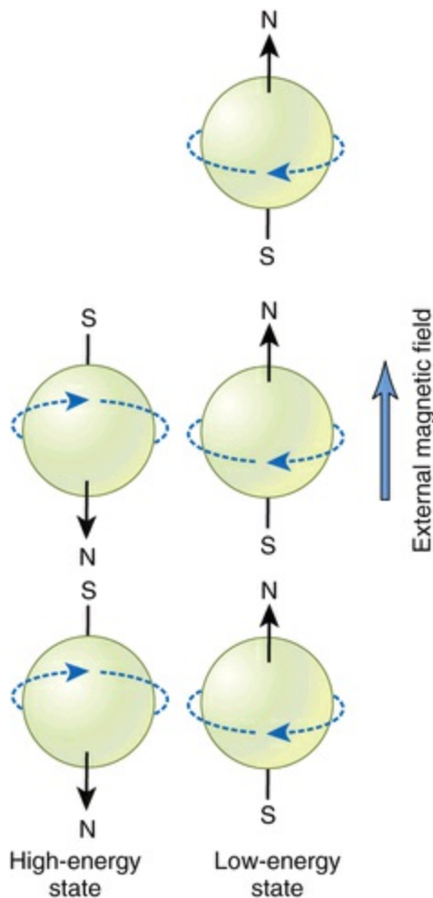
FIG. 13.14 Hydrogen Nuclei in an External Magnetic Field. In the presence of an applied strong external magnetic field, most nuclei are in the lower energy state and are aligned parallel with the magnetic field, whereas others align in the higher energy state antiparallel to the magnetic field.
