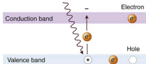
FIG. 4.5 X-ray or light photons impart energy to electrons in the valence band, releasing them into the conduction band. This generates an “electron hole” charge pair.
