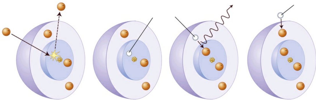
FIG. 1.14 Production of characteristic radiation. An incident electron (A) ejects an electron from an inner orbital creating an electron vacancy (B). (C) An electron from an outer orbital fills this vacancy, and a photon is emitted with energy equal to the difference in energy levels between the two orbitals. (D) Electrons from various orbitals may be involved, giving rise to other characteristic photons. The energies of the photons released are characteristic of the energy transitions for the target atom.
