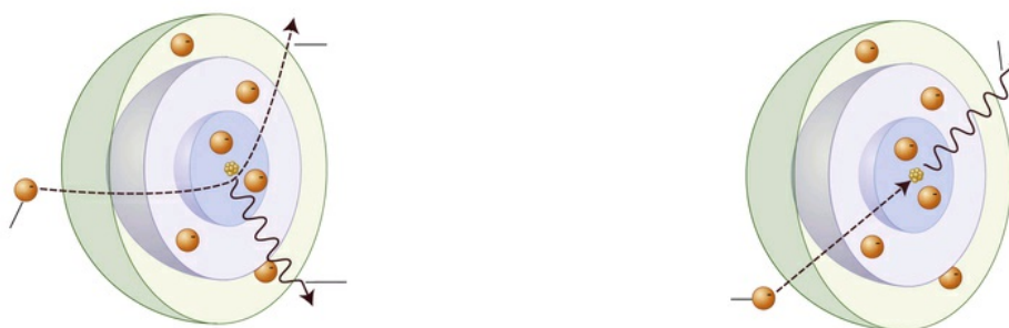
FIG. 1.12 Bremsstrahlung radiation is produced most often by the passage of an electron near a nucleus, which results in electrons being deflected and decelerated (A) or, less frequently, by the direct hit of an electron on a nucleus in the target (B). For the sake of clarity, this diagram and other similar figures in this chapter show only the 1s, 2s, or 3s orbitals.
