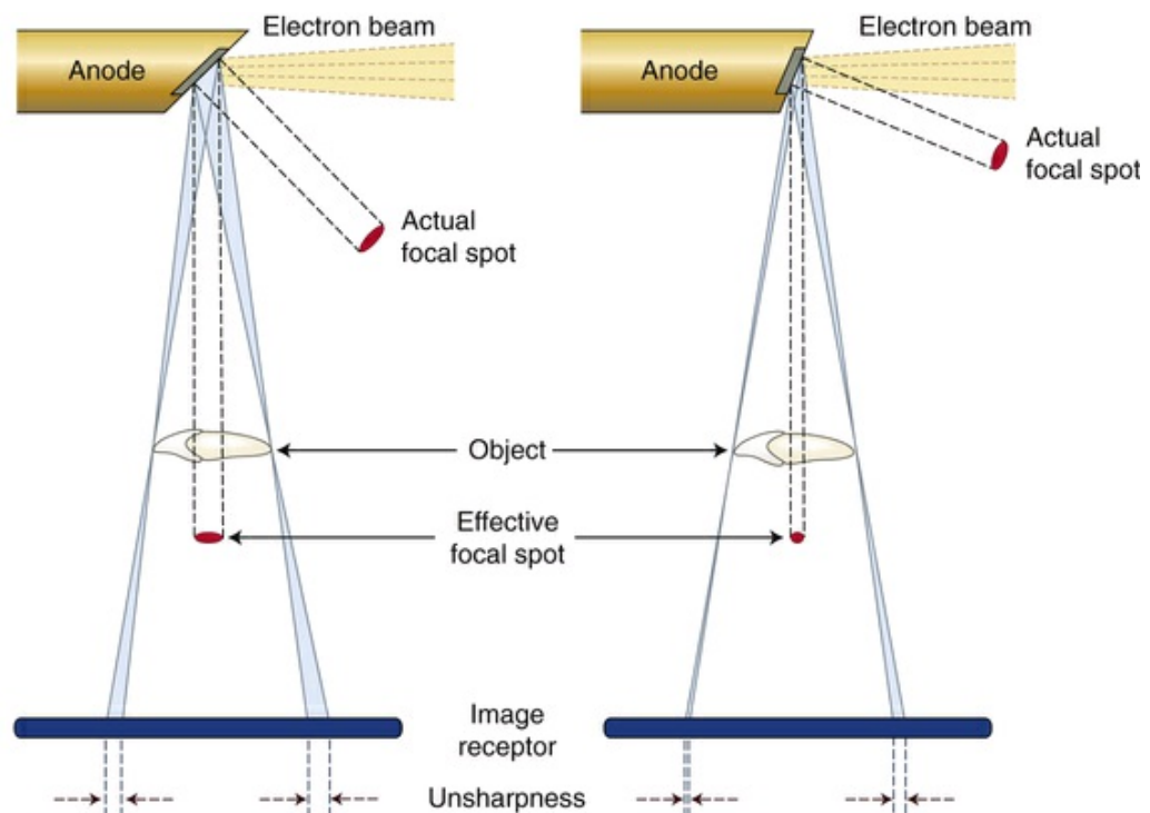
FIG. 6.2 As the angle of the target becomes closer to perpendicular to the long axis of the electron beam (as shown on the right ) the actual focal spot becomes smaller, which decreases heat dissipation and tube life. The more perpendicular angle also decreases the effective focal spot size, increasing the sharpness of the resulting image.
