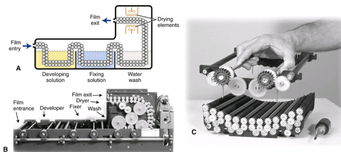
FIG. 5.21 (A) Automatic film processors typically consist of a roller assembly that transports the film through developing, fixing, washing, and drying stations. (B) Assembly of film transport mechanism. (C) One roller assembly. (B and C, Courtesy ImageWorks, Elmsford, NY.)
